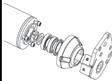
PROFESSIONAL REAR ROLLER Ø 140 mm (optional) with 4 taper roller bearings, mud scraper and interchangeable central body.
